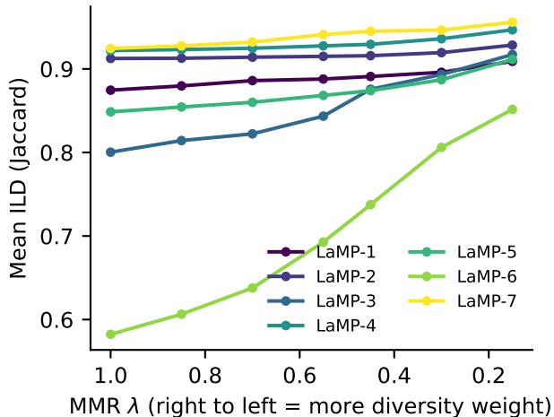
\lambda \rightarrow ILD (flan-T5-base (250M) / BM25)
