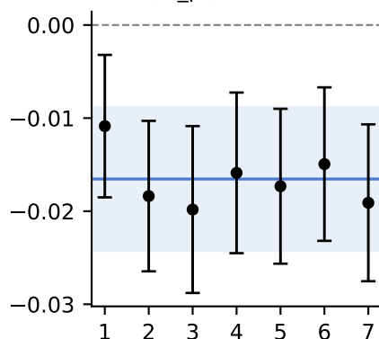
PL residual vs MMR coef(is_pl), ILD matched
