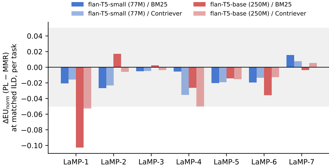
PL vs MMR utility at matched diversity, per task: small, mostly negative residuals
