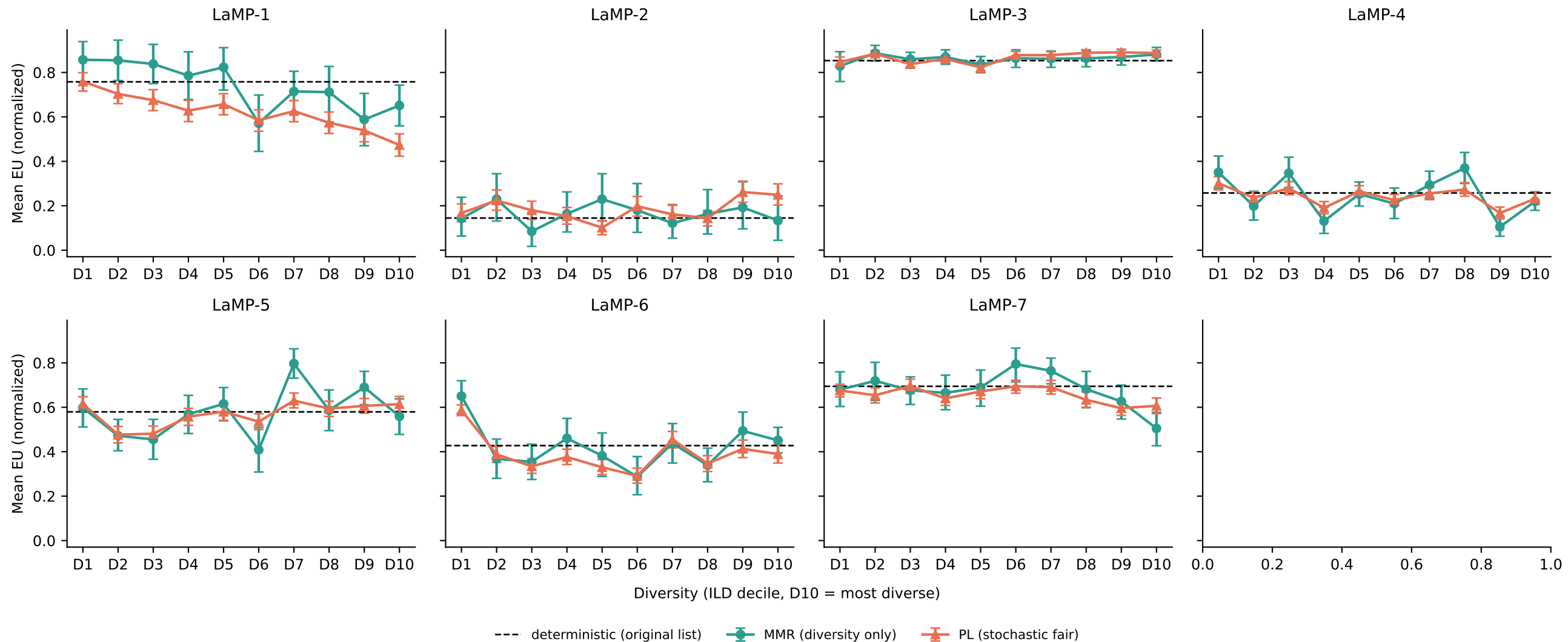
flan-T5-base (250M) / BM25: utility by diversity level, per LaMP task MMR vs PL vs the original deterministic list
