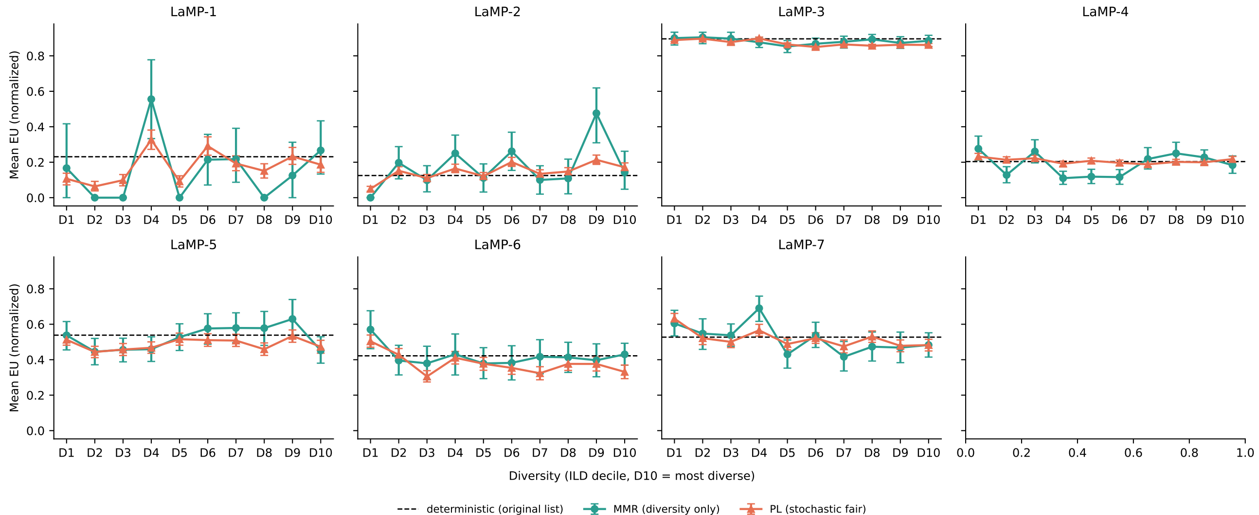
flan-T5-small (77M) / BM25: utility by diversity level, per LaMP task MMR vs PL vs the original deterministic list
