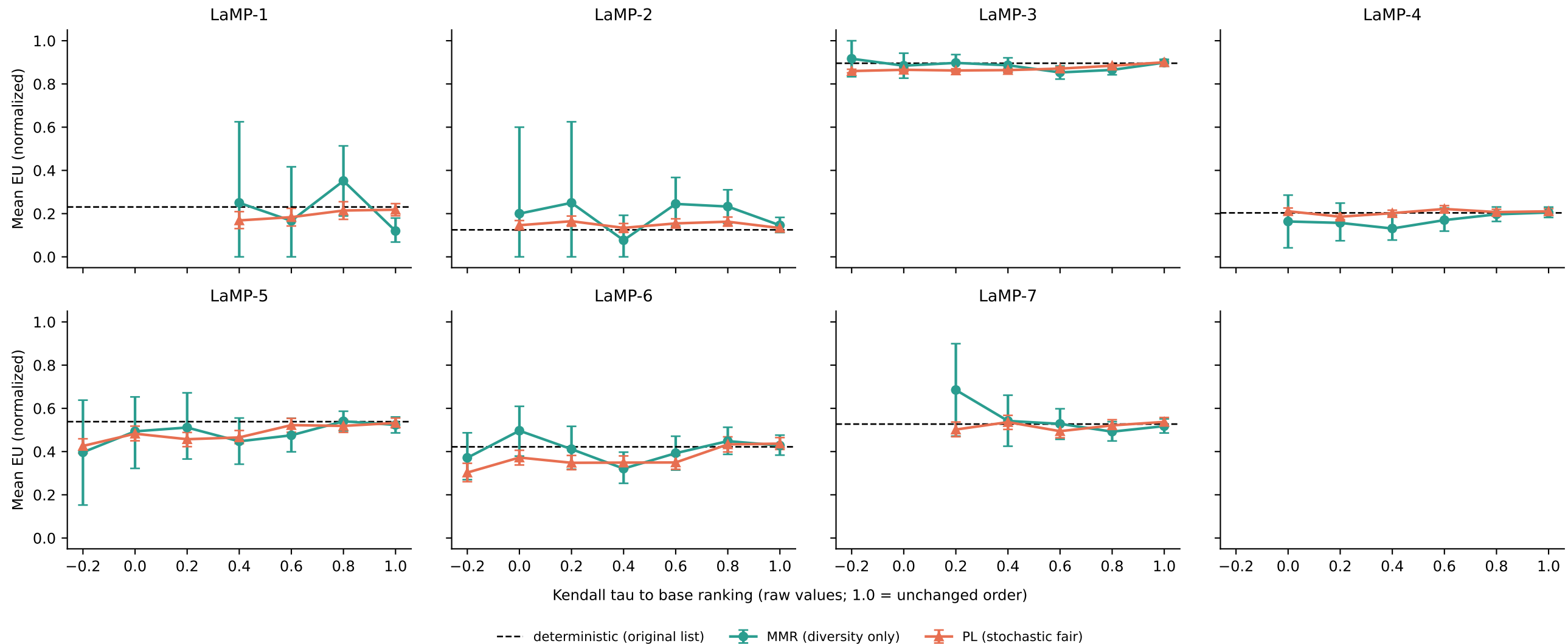
flan-T5-small (77M) / BM25: utility by how much a list reordered the base ranking (Kendall tau), per LaMP task MMR vs PL vs the original deterministic list
