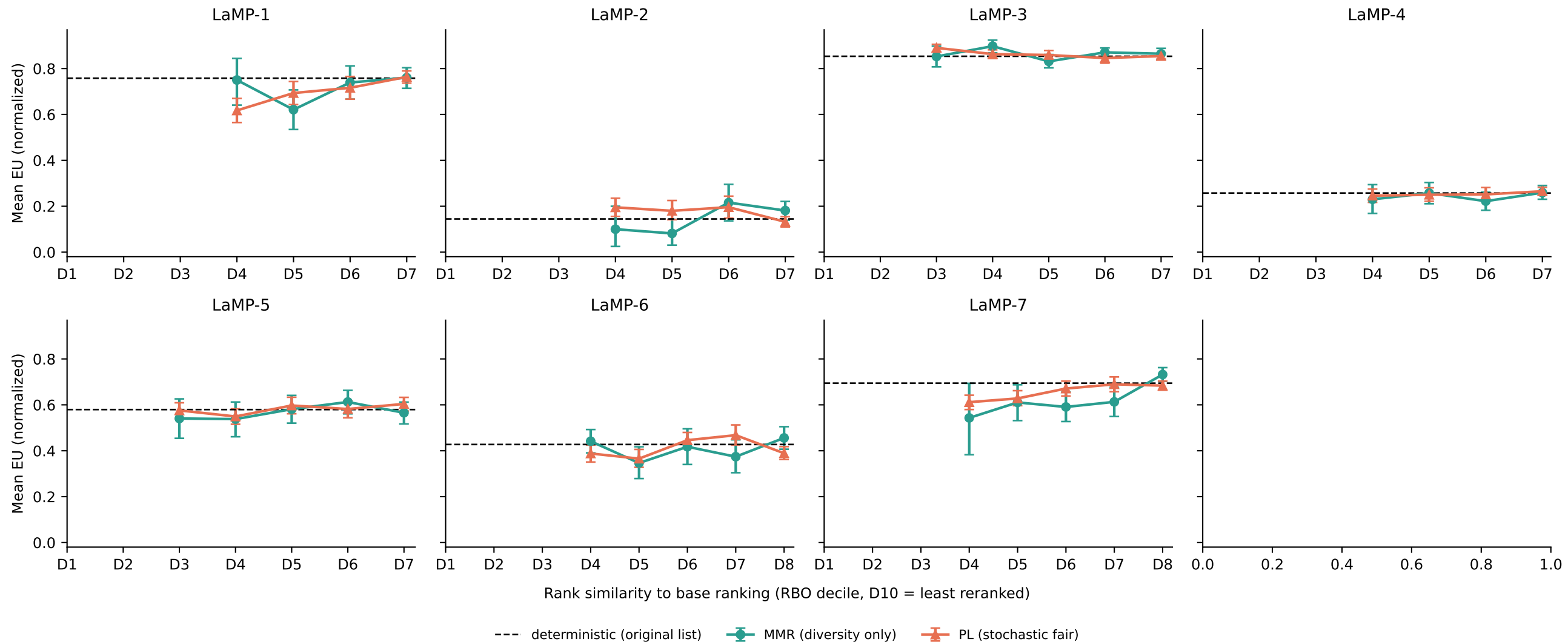
flan-T5-base (250M) / BM25: utility by how much a list reordered the base ranking (RBO), per LaMP task MMR vs PL vs the original deterministic list
