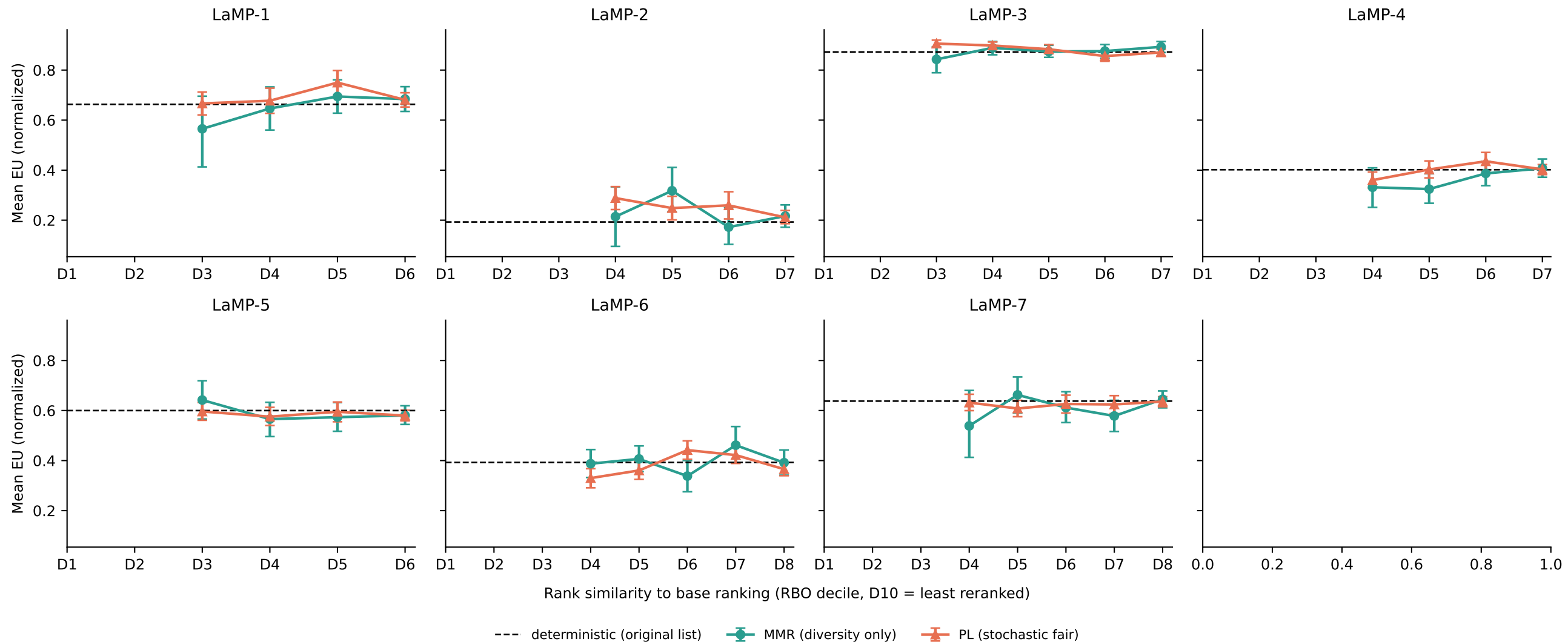
flan-T5-base (250M) / Contriever: utility by how much a list reordered the base ranking (RBO), per LaMP task MMR vs PL vs the original deterministic list
