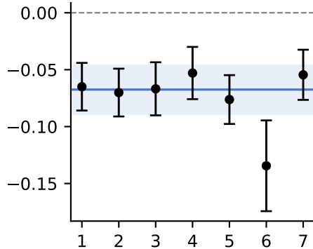
Finding 3: diversity effect coef(ILD), MMR rows only
