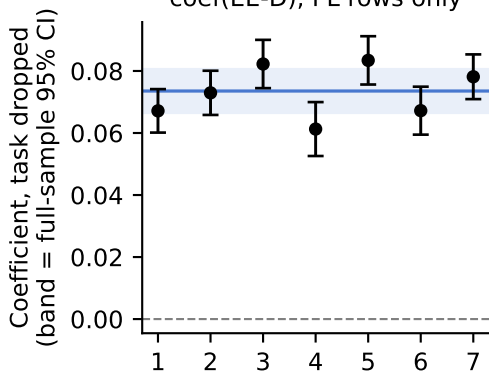
Finding 2: fairness-utility tradeoff coef(EE-D), PL rows only
