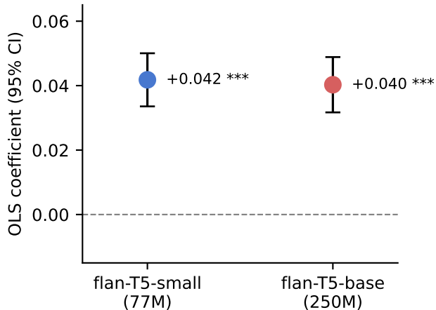
M2: fairness cost of exposure equality coef(EE-D) on EU_{norm} , controlling ILD
