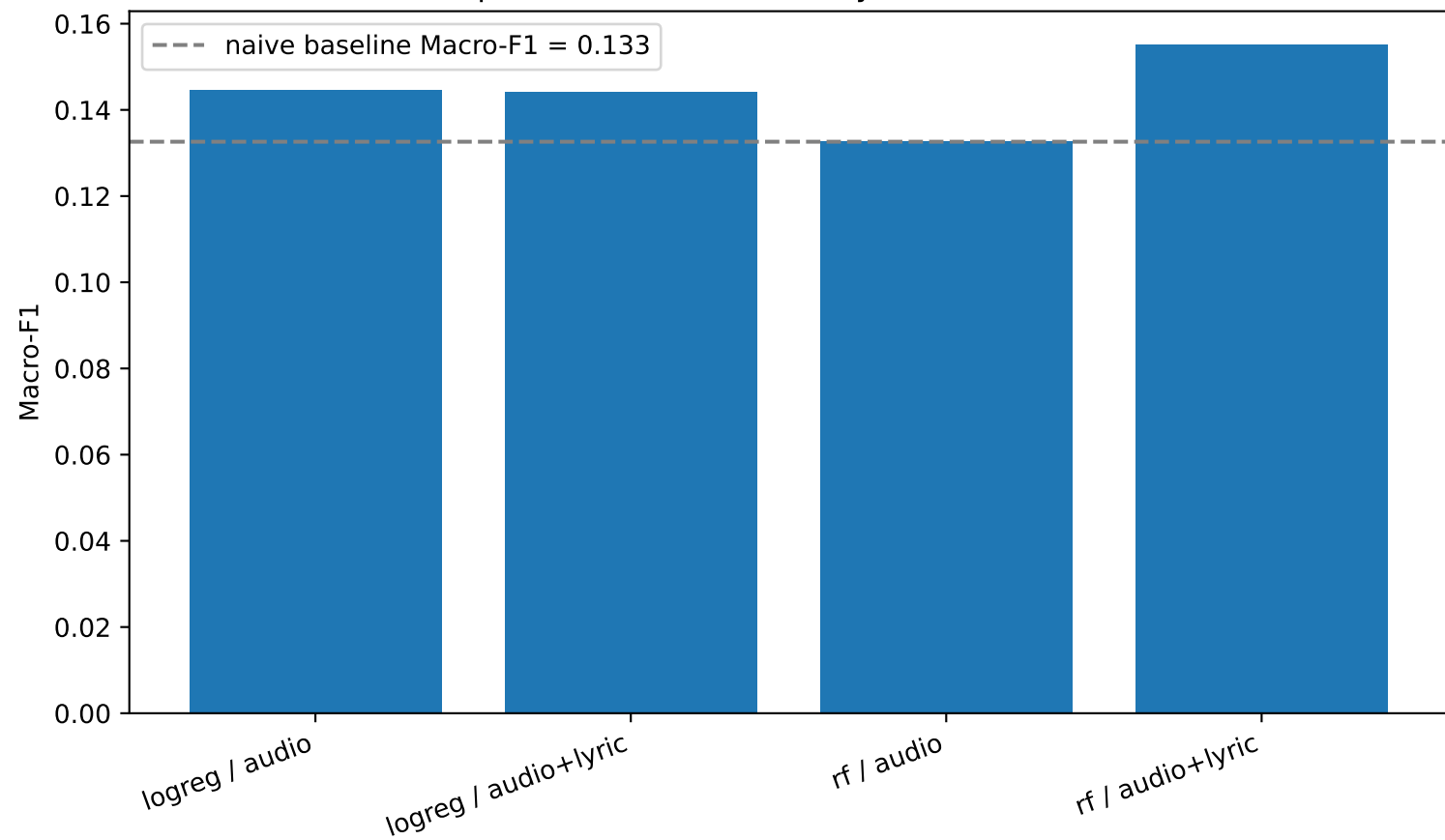
Decade prediction — Macro-F1 by model and feature set
