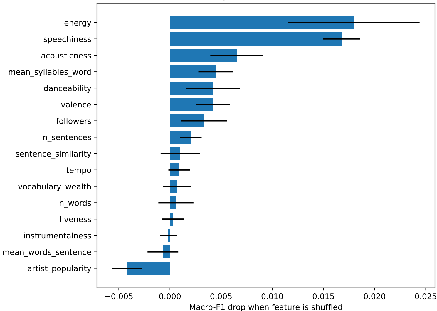
Permutation importance — tuned Random Forest
