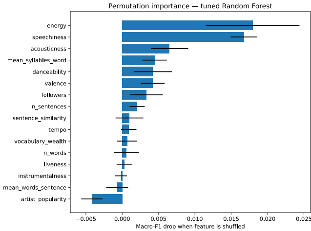
Fig. 3. Permutation importance for the tuned Random Forest, scored by macro-F1 drop. Error bars are standard deviations over 10 permutations.
