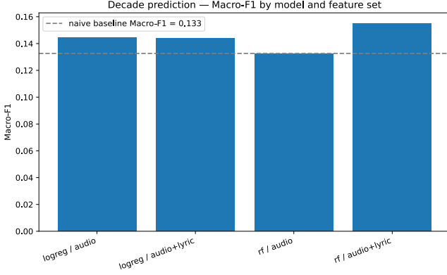
Fig. 2. Macro-F1 by model and feature set. Dashed line is the naive baseline.
