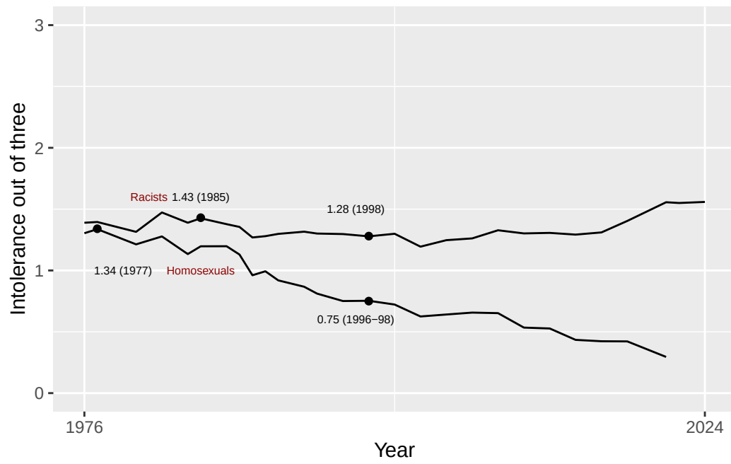
Figure 5 extended
