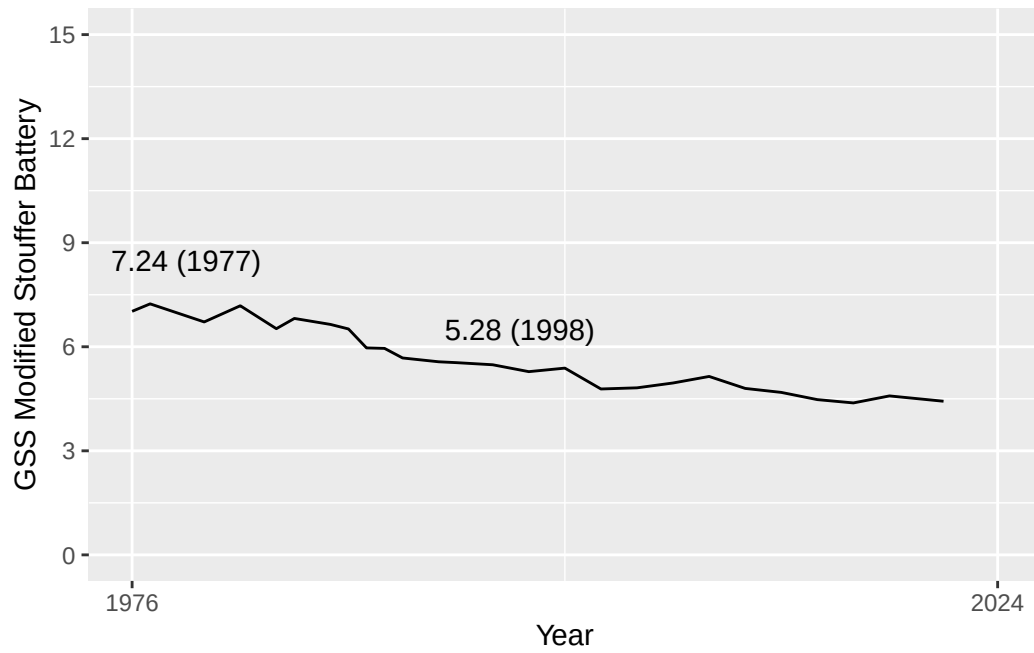
Figure 2 Extended
