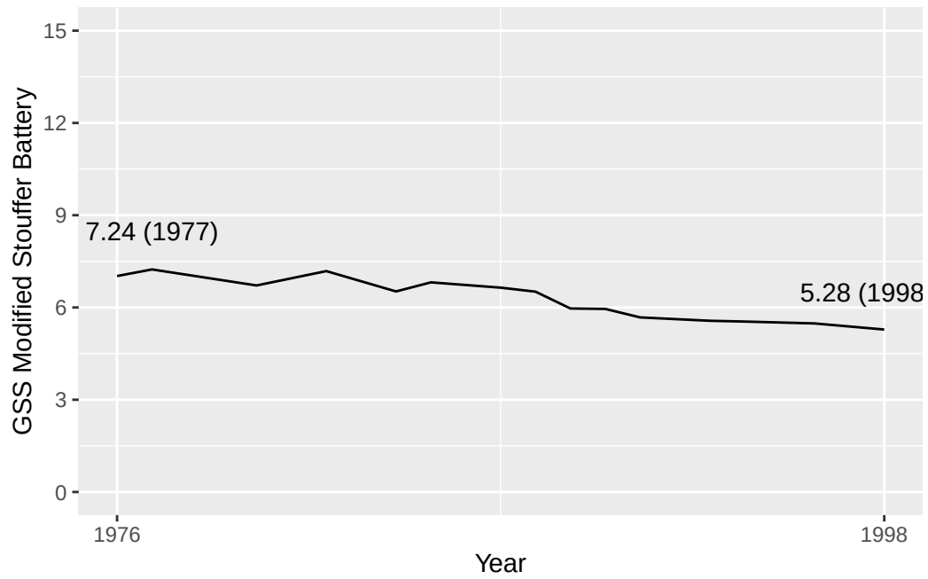
Figure 2 Replication
