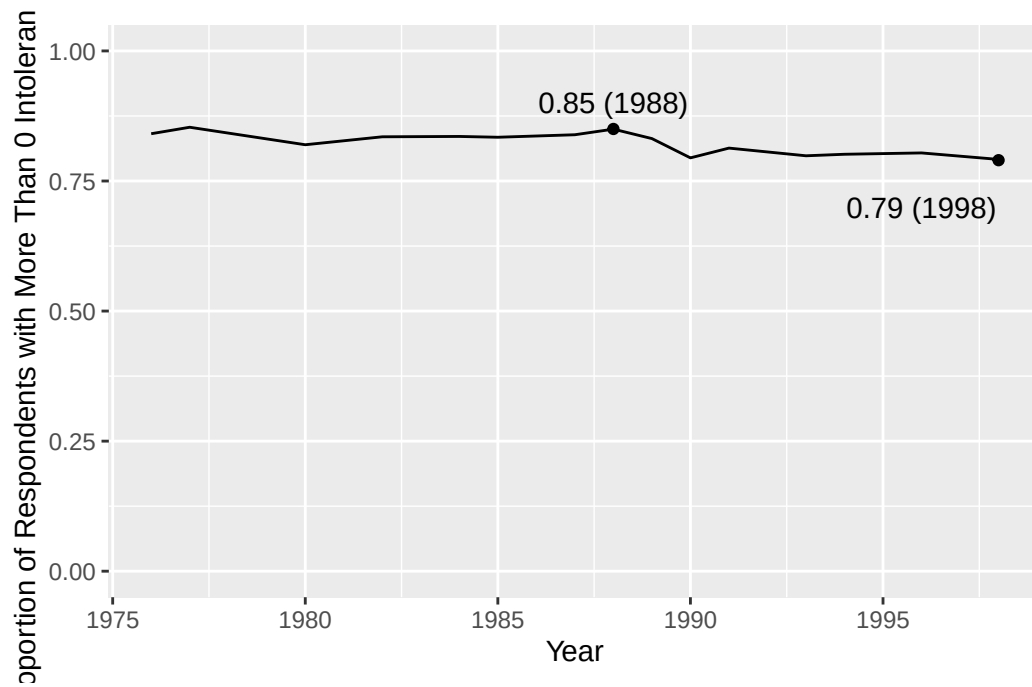
Figure 5 Replication
