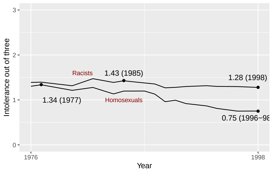
Figure 2 Replication
