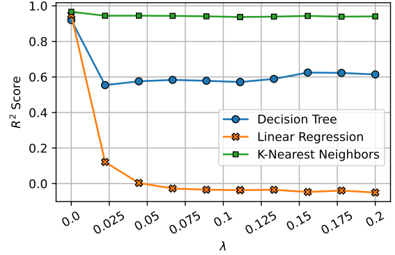
Figure 1: Effect of the baseline-penalization parameter \lambda on model performance. The figure reports the R^2 score of different regression models as \lambda increases.
