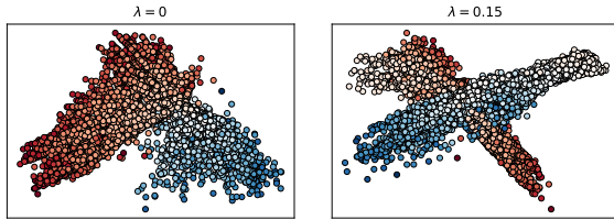
Figure 4: Effect of the baseline penalty on dataset structure. Two-dimensional PCA projections of datasets generated with the proposed method for \lambda = 0 (left) and \lambda = 0.15 (right).
