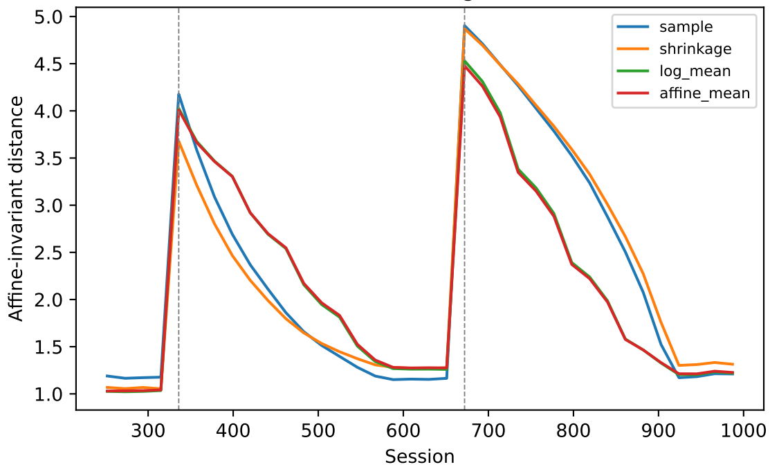
Covariance error and regime transitions
