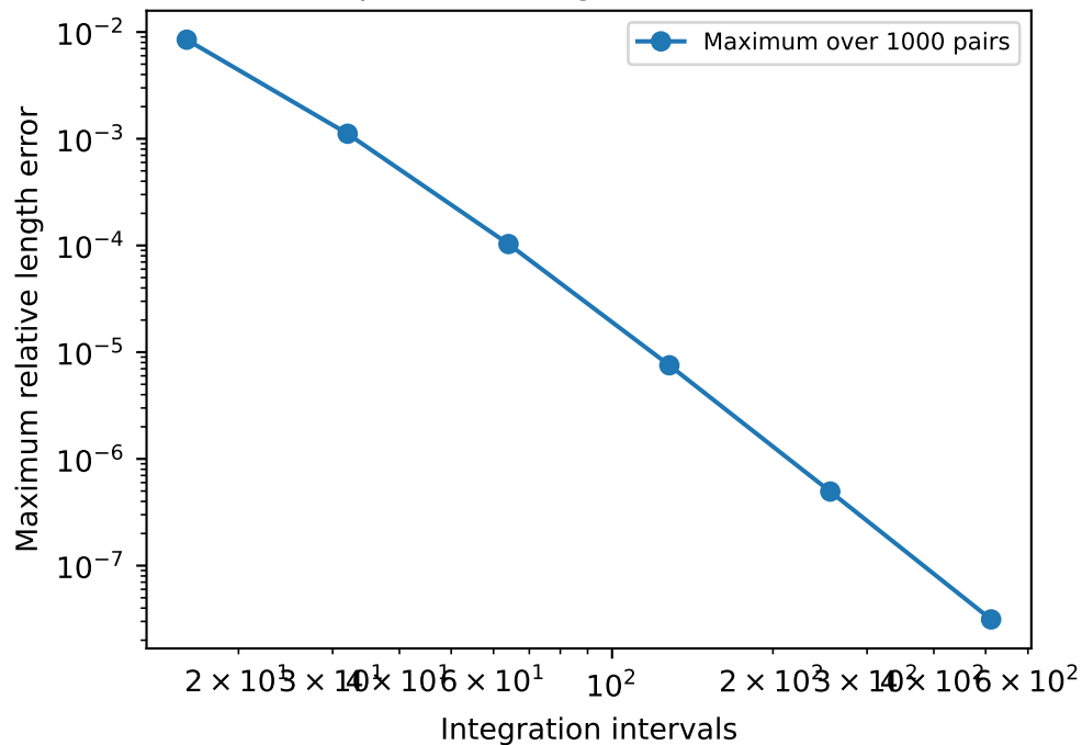
Simpson convergence: order 3.90
