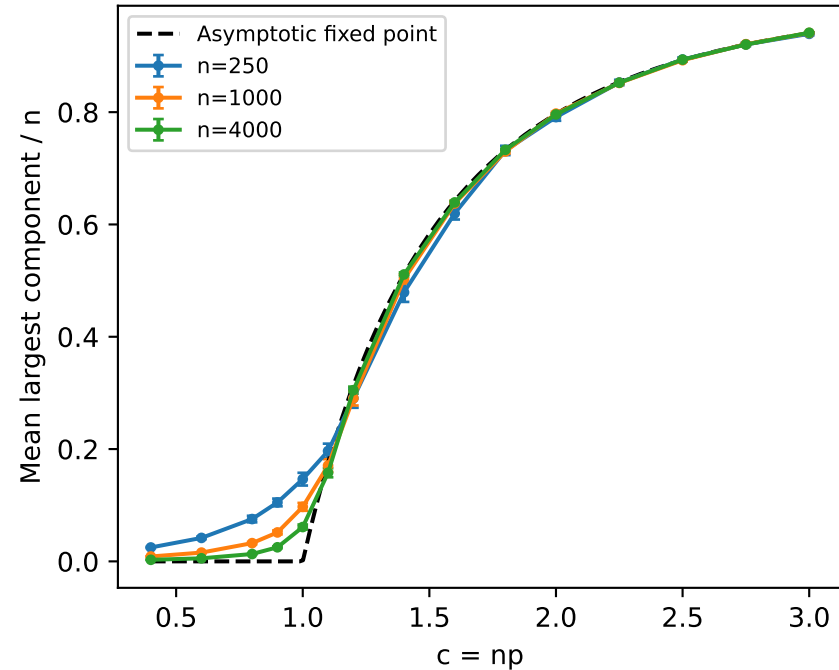
Giant-component transition
