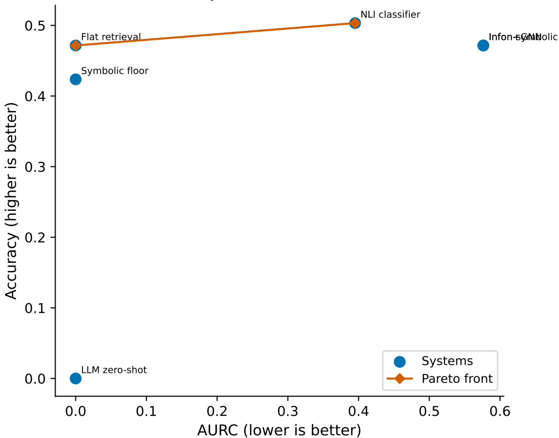
Accuracy vs AURC — Pareto front
