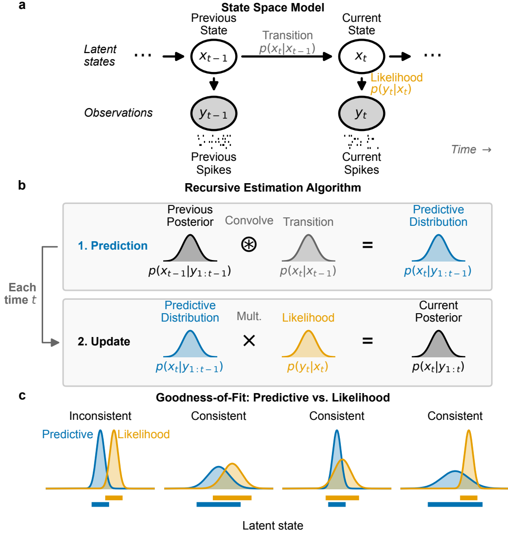
Fig 1. State-space model and local goodness-of-fit measures. (a) The graphical representation of the state-space model includes the state transition model, p(x_k | x_{k-1}) , and the observation likelihood p(y_k | x_k) . (b) These model components are sufficient to compute an iterative expression for the filtering distribution at time t_k , p(x_k | y_{1:k}) , from the distribution at the previous time step. This involves first convolving the previous posterior with the state transition distribution to compute the one-step predictive distribution, p(x_k | y_{1:k-1}) , and then updating the predictive distribution with information from the most recent spiking by multiplying by the observation likelihood. (c) For each new spike observation, we compute the local goodness-of-fit by assessing the consistency of information between the predictive distribution and likelihood. We consider the distributions inconsistent when they assign high probability to mostly disjoint subsets of the state space. When the regions with high probability overlap, the distributions are considered consistent, even if the distributions differ in their central tendency or certainty.
