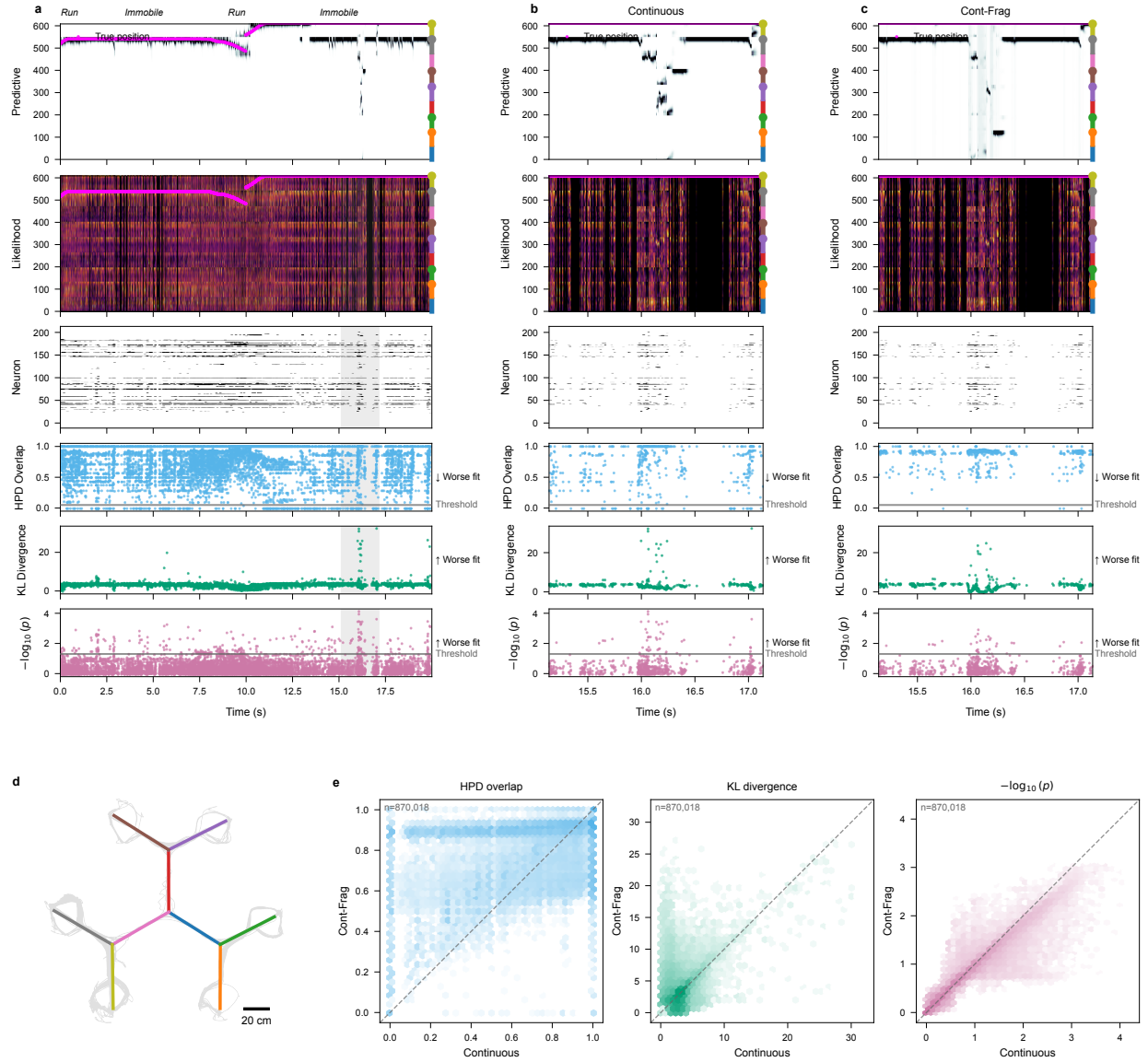
Figure 4: Per-spike goodness-of-fit diagnostics applied to a real hippocampal recording (203 simultaneously recorded cells) during navigation on a multi-arm maze; data from Comrie et al. [2024] . Two state-space decoders—a purely Continuous decoder and a Continuous–Fragmented decoder—are evaluated on the same session. (a) Wider context window under the Continuous decoder; behavioral periods (Run / Immobile) are labeled along the top axis, and the shaded band marks the zoom window shown in (b) and (c) . (b) , (c) The same zoom window decoded with the Continuous and Continuous–Fragmented decoders, respectively. Within each column of (a) – (c) , all rows share a common time axis ( x , seconds, relative to the start of the context window). Row 1, Predictive : heatmap of the predictive posterior with linearized position on y and the animal’s true linearized position overlaid. Row 2, Likelihood : same axes, restricted to time bins containing at least one spike, showing the combined per-spike likelihood. Row 3, Neuron : spike raster with neurons on y , sorted by place-field peak position. Rows 4–6 (HPD overlap, KL divergence, -\log_{10}(p) ) : one marker per spike event placed at its spike time, with the per-spike diagnostic value on y ; a horizontal dashed line marks the threshold used to flag poor model fit, and the direction of worse fit is labeled at the right. (d) 2D layout of the track with the animal’s trajectory overlaid in grey and a 20 cm scale bar. (e) Pairwise comparison of per-spike diagnostic values between the two decoders across the whole session, one hexbin panel per metric (HPD overlap, KL divergence, -\log_{10}(p) ); x -axis is the Continuous decoder, y -axis is the Continuous–Fragmented decoder, and the dashed line is identity. Hexagons are coloured by spike-event density (log scale).
