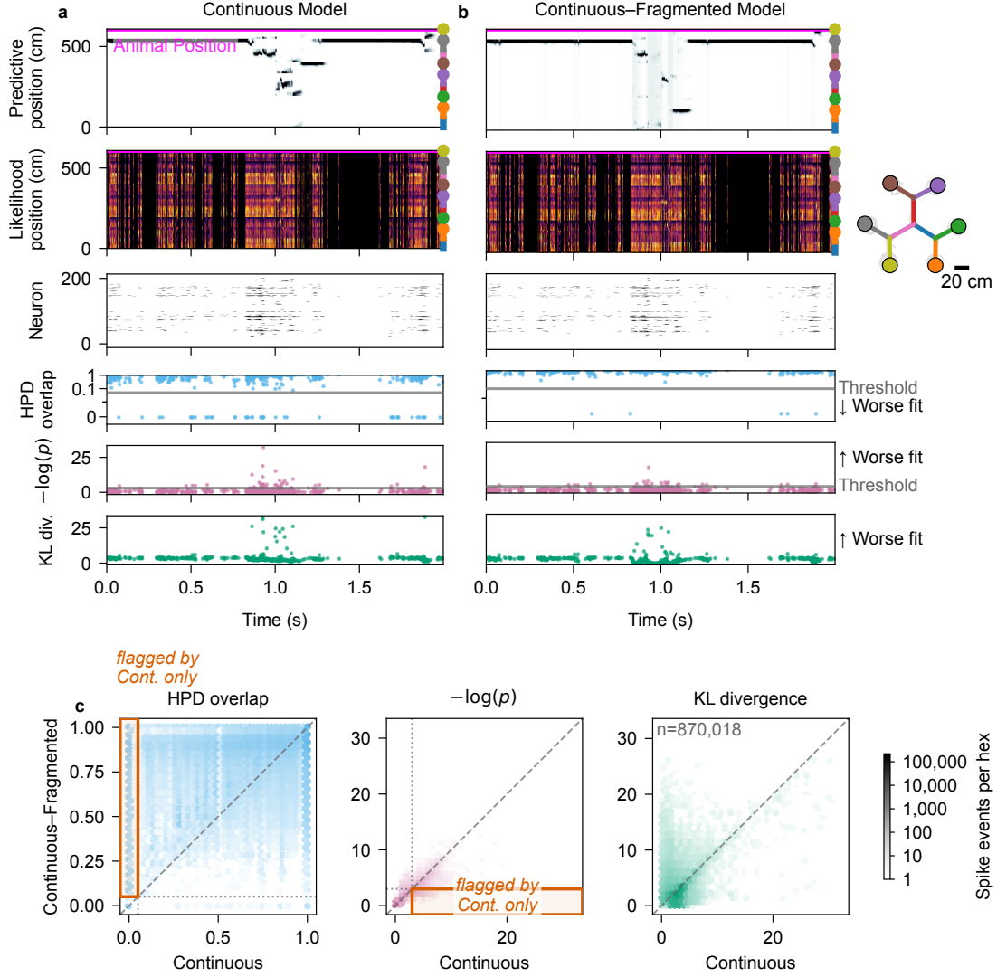
Fig 4. Per-spike goodness-of-fit diagnostics applied to a hippocampal recording of 203 simultaneously recorded units during navigation on a multi-arm maze (data from Comrie et al. [17]), evaluated under a Continuous and a Continuous-Fragmented state-space model. The inset shows the two-dimensional maze with the animal's trajectory in gray; colored dots mark the six reward wells. (a, b) A window containing a candidate replay event, decoded with the Continuous (a) and Continuous-Fragmented (b) models; time is relative to the start of the window. Row 1: the one-step predictive distribution over linearized position, with the animal's physical position overlaid; the Continuous-Fragmented model's dynamics mode is marginalized. Row 2: the mean normalized per-spike likelihood, identical under both models. Row 3: the spike raster, with units sorted by place-field peak position. Rows 4–6: HPD overlap, -\log(p) , and KL divergence for each spike event. Horizontal lines mark the flag cutoff of 0.05 for HPD overlap and the predictive p -value (the latter shown as -\log(0.05) \approx 3 ); KL divergence has no fixed cutoff. (c) Per-spike diagnostic values across the session under the Continuous (x-axis) and Continuous-Fragmented (y-axis) models; the dashed line is the identity and dotted lines mark flag thresholds. The outlined box contains spikes flagged only under the Continuous model. Color gives the number of spike events on a shared logarithmic scale.
