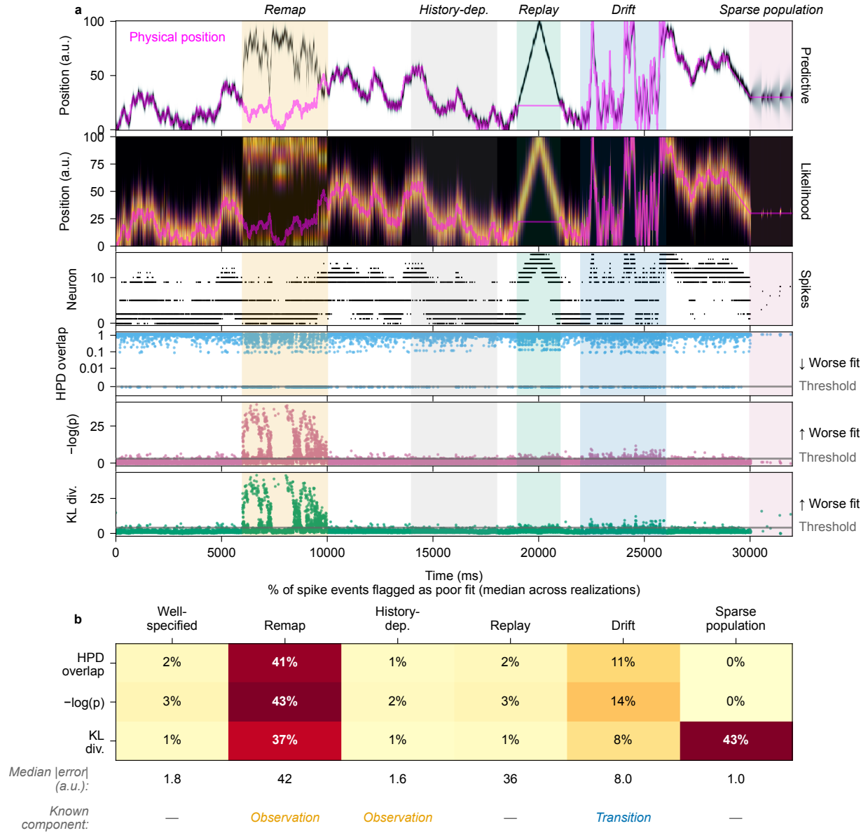
Fig 3. Per-spike goodness-of-fit diagnostics for the simulation study. (a) Top row: the predictive distribution over time and position, with the animal’s physical position in magenta; shading marks the three misfit periods and two controls. Second row: the mean normalized per-spike likelihood in each spike-containing bin. Third row: the spike raster, with neurons sorted by place-field peak position. Bottom rows: HPD overlap (symmetric-log axis), the rank-based predictive p -value, and KL divergence for each spike event, with flag thresholds. (b) Median percentage of spike events flagged in each phase across 100 realizations, with clean-recovery windows pooled into one column. HPD and KL thresholds come from the pooled opening baseline (steps 0–6,000); the predictive p -value uses a fixed cutoff of 0.05. The decoding-error row gives the median absolute error (a.u.) of the filtered posterior mean relative to the true position, which in the replay column is the animal’s fixed physical position, so the error is large by construction. The bottom row names the perturbed component ( Observation or Transition ); a dash marks well-specified and control phases.
