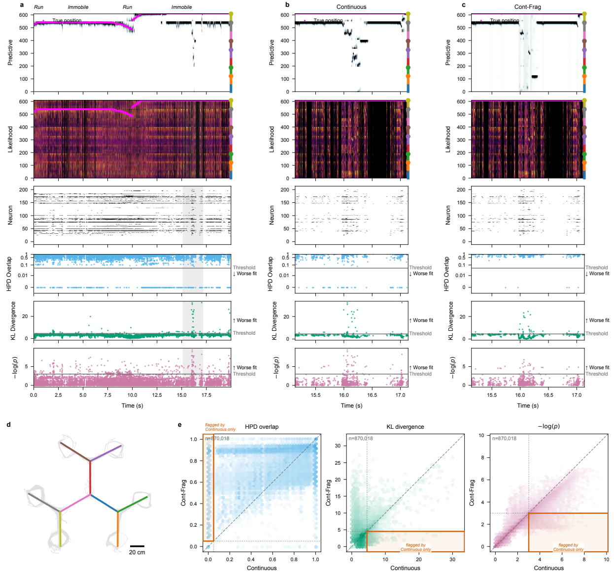
Figure 4: Per-spike goodness-of-fit diagnostics applied to a real hippocampal recording (203 simultaneously recorded cells) during navigation on a multi-arm maze; data from ?. Two state-space decoders—a purely Continuous decoder and a Continuous-Fragmented decoder—are evaluated on the same session. (a) Wider context window under the Continuous decoder; behavioral periods (Run / Immobile) are labeled along the top axis, and the shaded band marks the zoom window shown in (b) and (c). (b), (c) The same zoom window decoded with the Continuous and Continuous-Fragmented decoders, respectively. Within each column of (a)–(c), all rows share a common time axis ( x , seconds, relative to the start of the context window). Row 1, Predictive: heatmap of the predictive posterior with linearized position on y and the animal's true linearized position overlaid. Row 2, Likelihood: same axes, restricted to time bins containing at least one spike, showing the combined per-spike likelihood. Row 3, Neuron: spike raster with neurons on y , sorted by place-field peak position. Rows 4–6 (HPD overlap, KL divergence, -\log(p) ): one marker per spike event placed at its spike time, with the per-spike diagnostic value on y ; a horizontal line marks the threshold used to flag poor model fit (HPD overlap and the predictive p -value at a fixed 0.05 cutoff; KL divergence at the 99th-percentile baseline threshold carried over from the simulation in Figure ??, \approx 4.52 ), and the direction of worse fit is labeled at the right. (d) 2D layout of the track, with the maze arms drawn as colored segments, the animal's trajectory overlaid in grey, and a 20 cm scale bar. (e) Pairwise comparison of per-spike diagnostic values between the two decoders across the whole session, one hexbin panel per metric (HPD overlap, KL divergence, -\log(p) ); x -axis is the Continuous decoder, y -axis is the Continuous-Fragmented decoder, and the dashed line is identity. Dotted lines mark the per-metric flag threshold on each axis (the same values used in panels (a)–(c)), and the outlined box marks the quadrant of spikes flagged by the Continuous decoder but not the Continuous-Fragmented decoder. Hexagons are colored by spike-event density (log scale).
