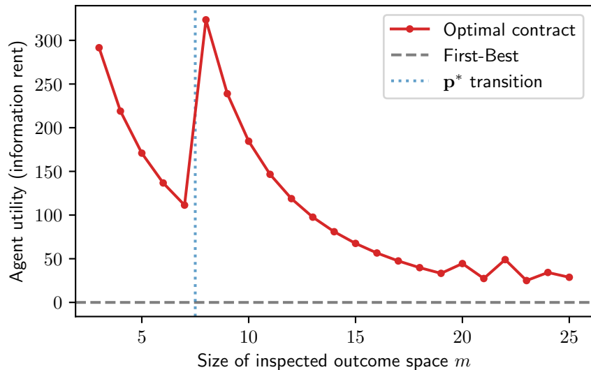
Agent Utility for Varying Outcome Informativeness
