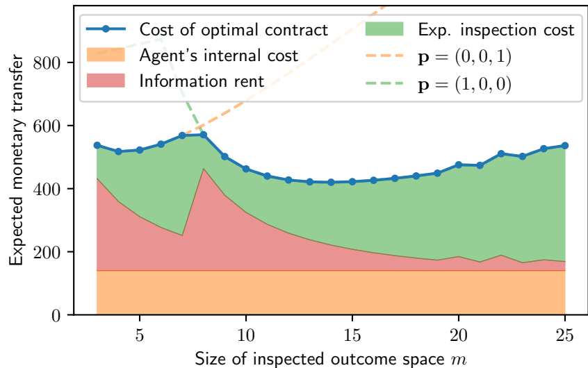
Contract Cost Breakdown for Varying Informativeness
