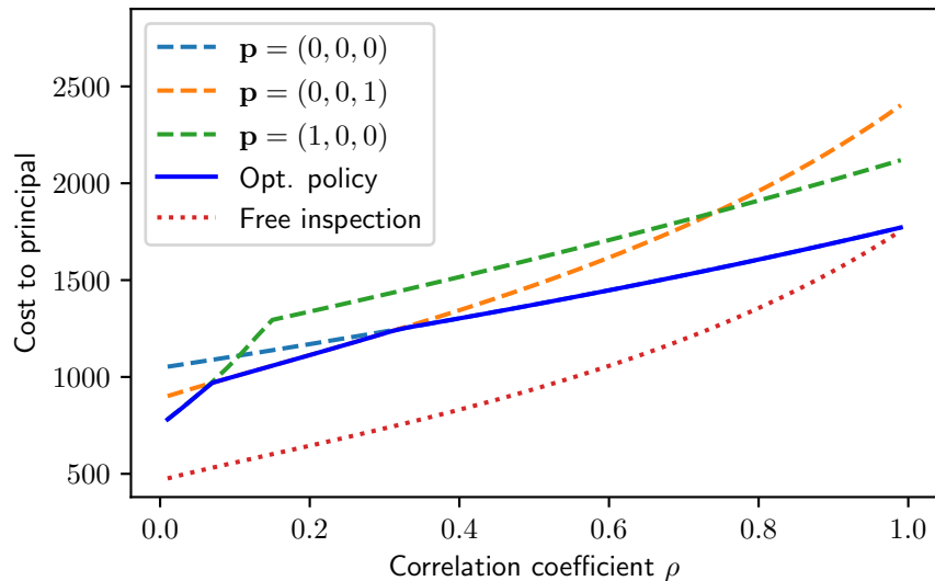
Expected Pay Under Beta-Binomial Correlation
