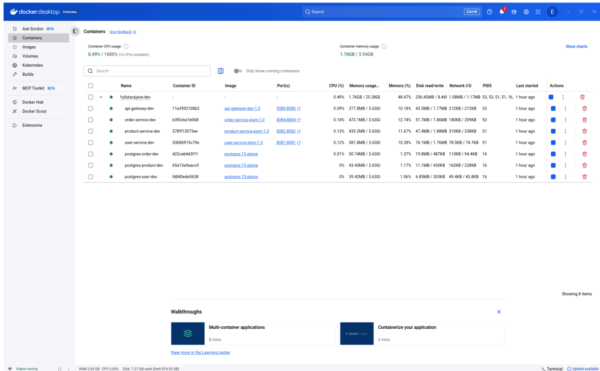
Figura 1 - Docker Desktop
