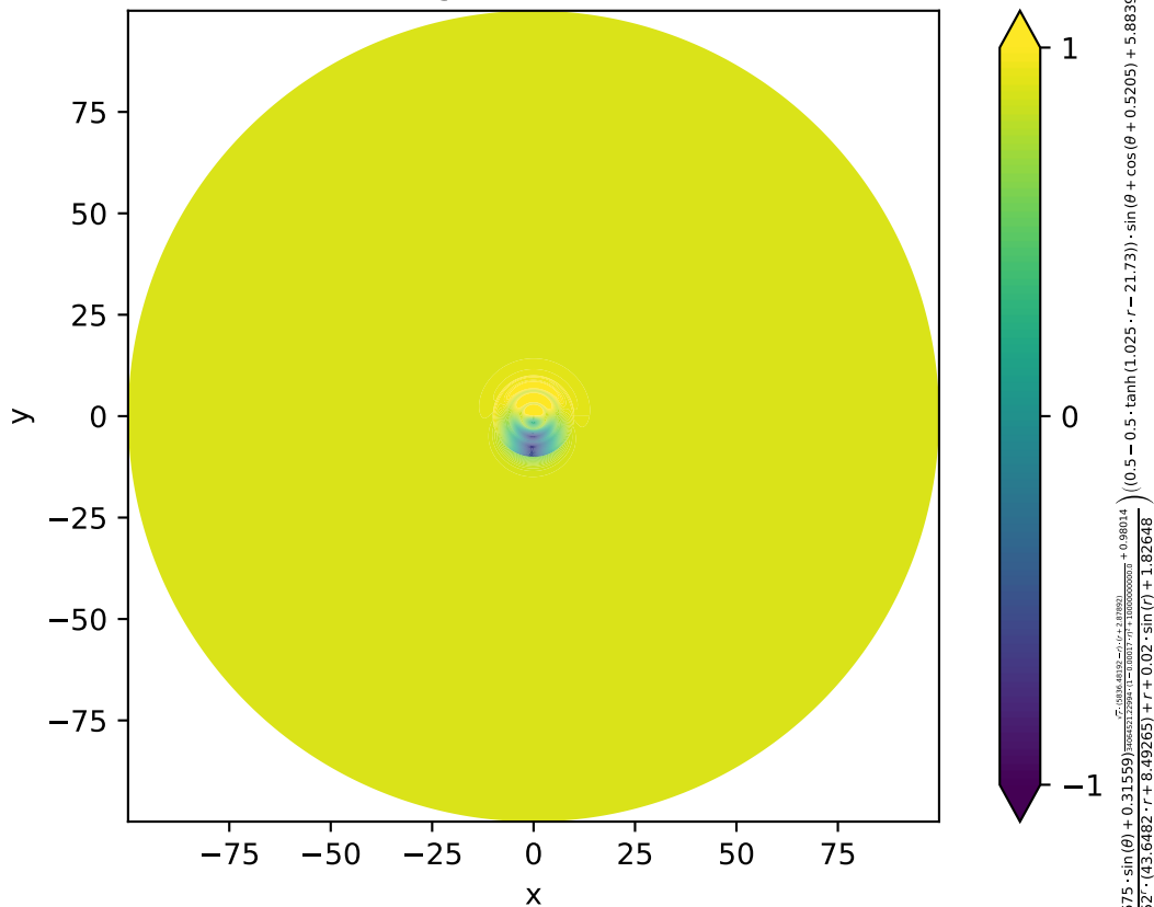
Swift-Hohenberg 2D Pattern, MSE = 0.009
