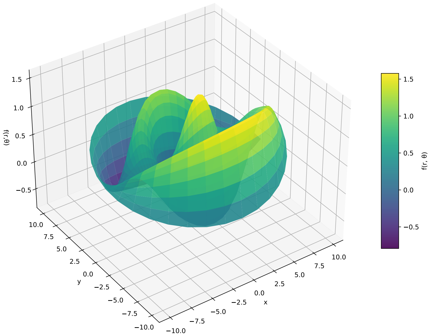
Swift-Hohenberg 2D Pattern (3D Surface)
