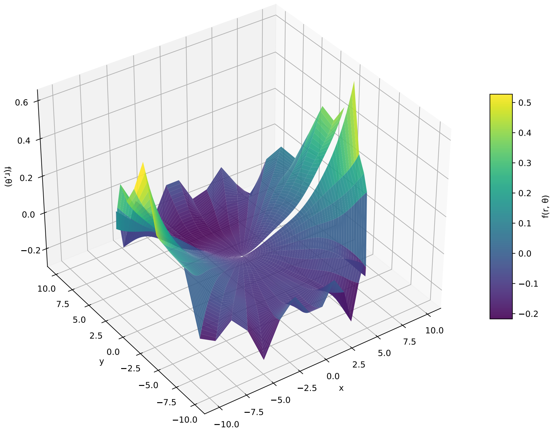
Swift-Hohenberg 2D Solution ( U^\star ) — 3D Surface
