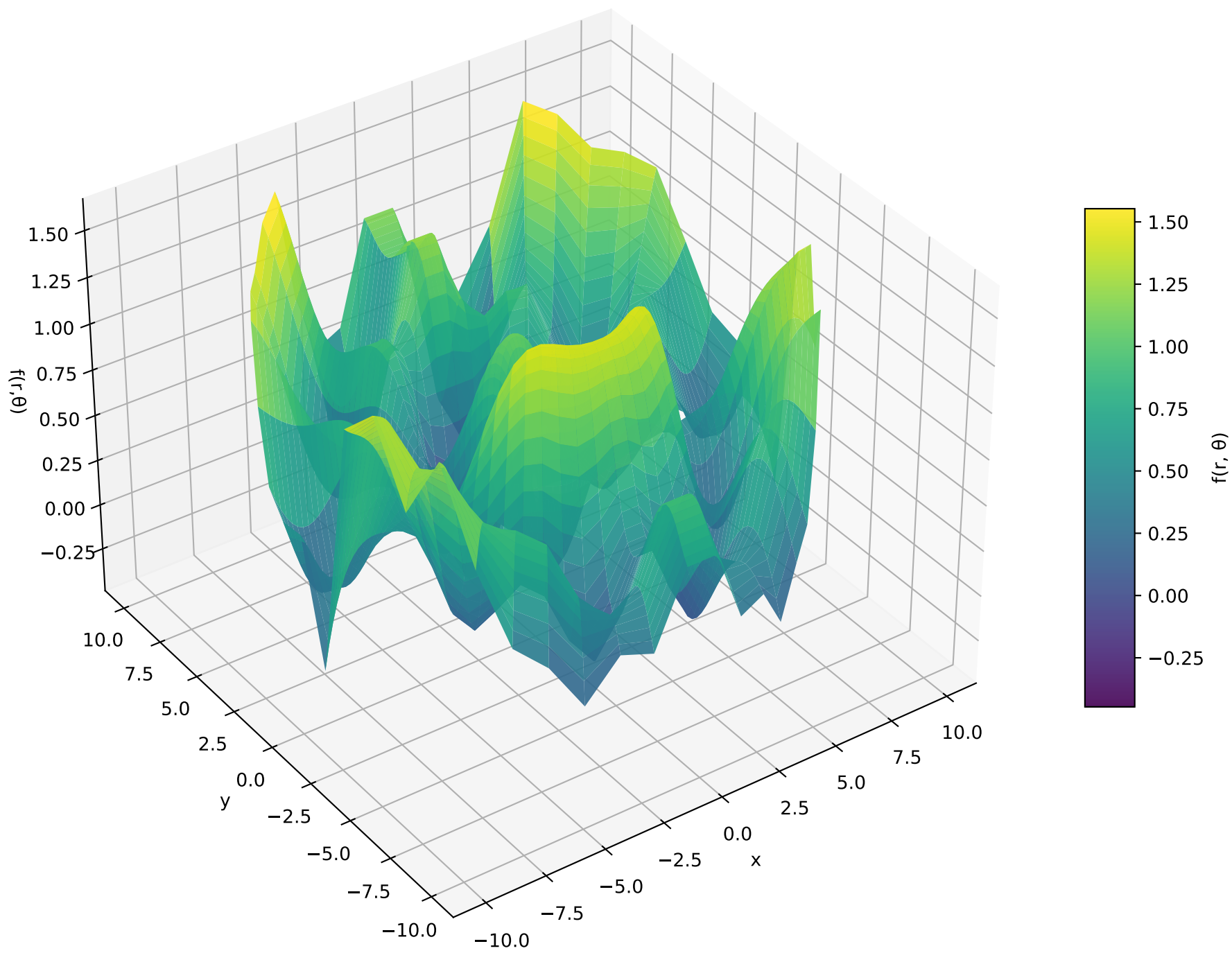
Swift-Hohenberg 2D Solution ( U^\star ) — 3D Surface
