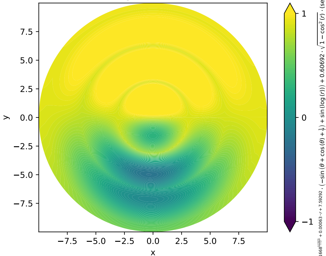
Swift-Hohenberg 2D Pattern, MSE = 0.026
