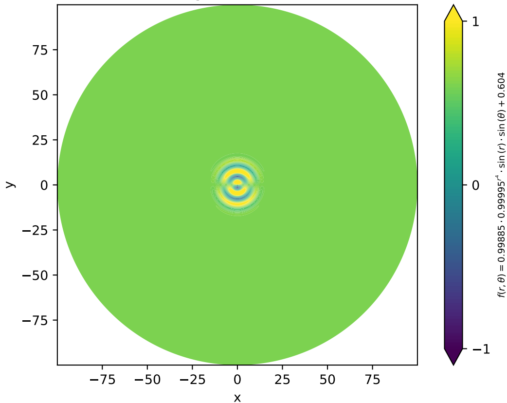
Swift-Hohenberg 2D Pattern, MSE = 0.032
