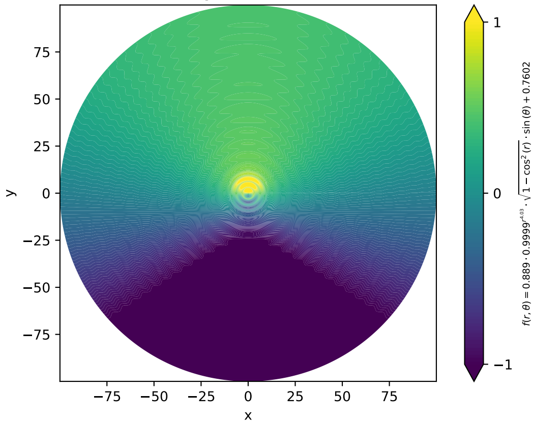
Swift-Hohenberg 2D Pattern, MSE = 0.025
