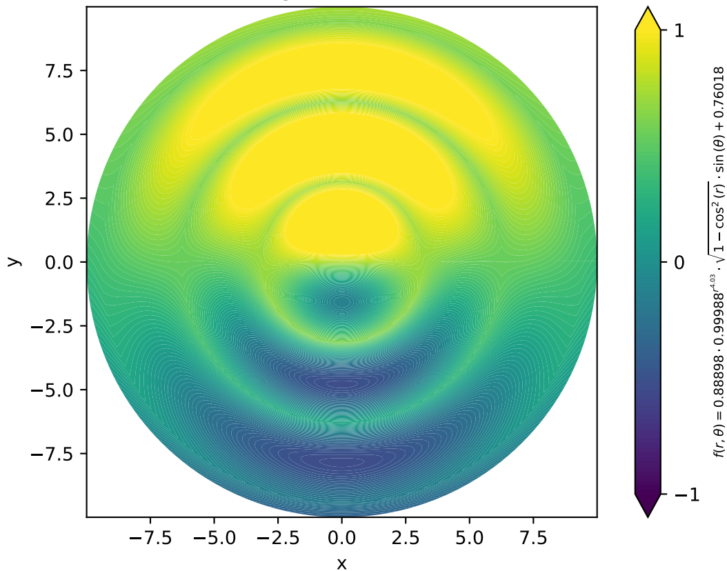
Swift-Hohenberg 2D Pattern, MSE = 0.078
