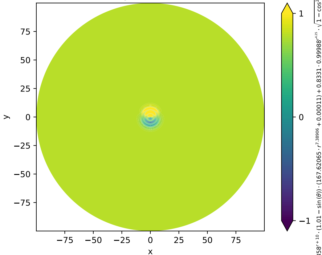
Swift-Hohenberg 2D Pattern, MSE = 0.022
