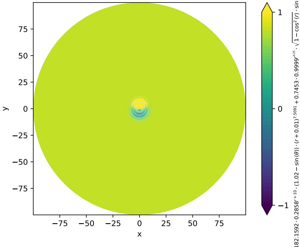
Swift-Hohenberg 2D Pattern, MSE = 0.019
