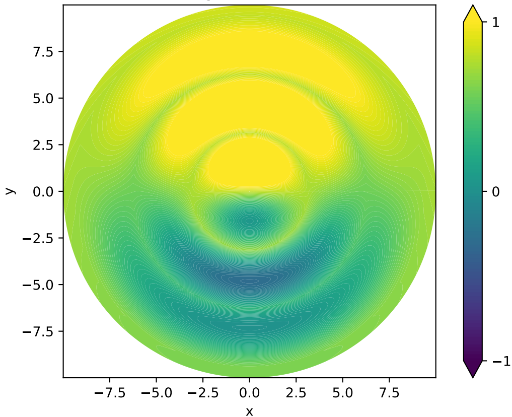
Swift-Hohenberg 2D Pattern, MSE = 0.047
