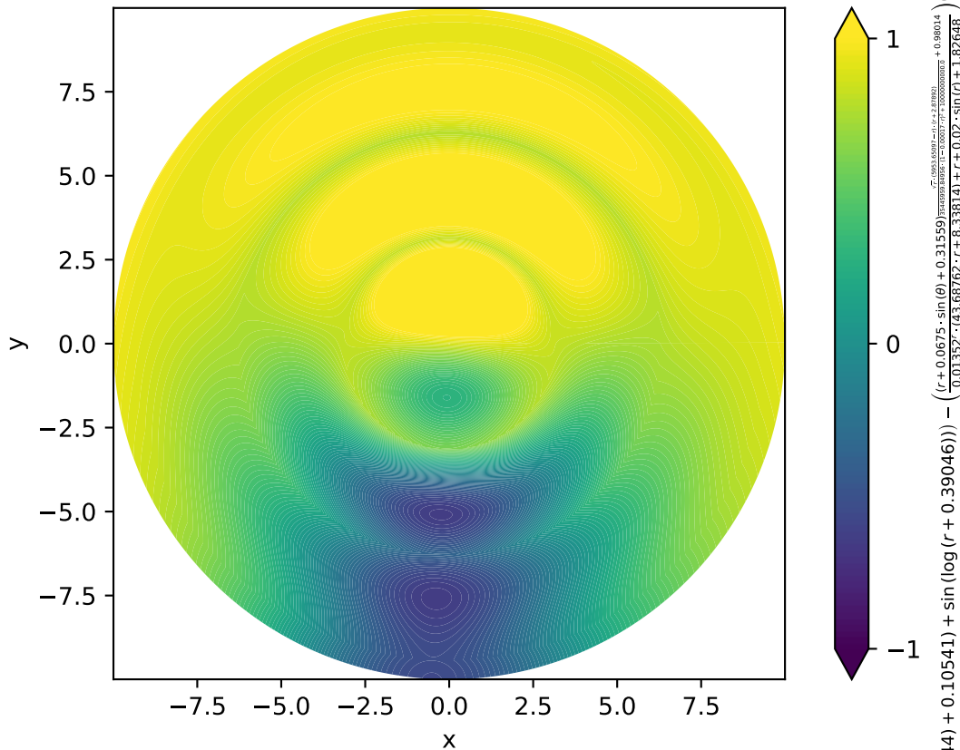
Swift-Hohenberg 2D Pattern, MSE = 0.015
