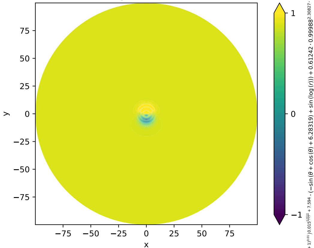
Swift-Hohenberg 2D Pattern, MSE = 0.011
