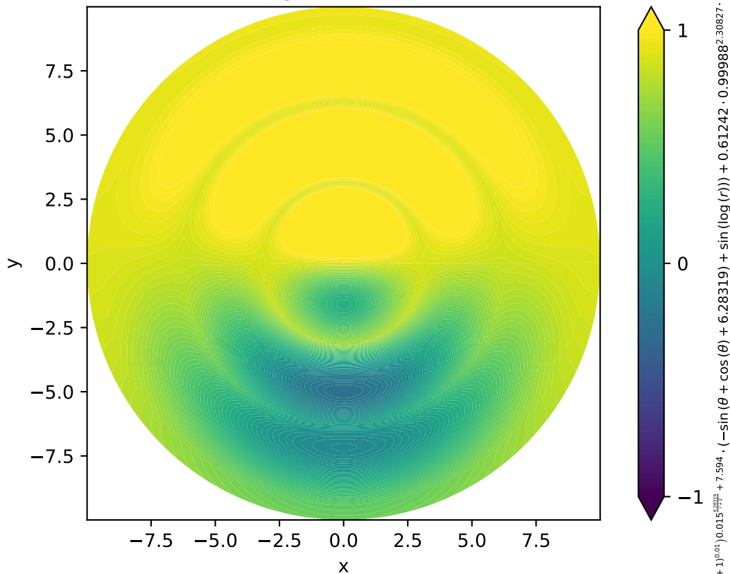
Swift-Hohenberg 2D Pattern, MSE = 0.027
