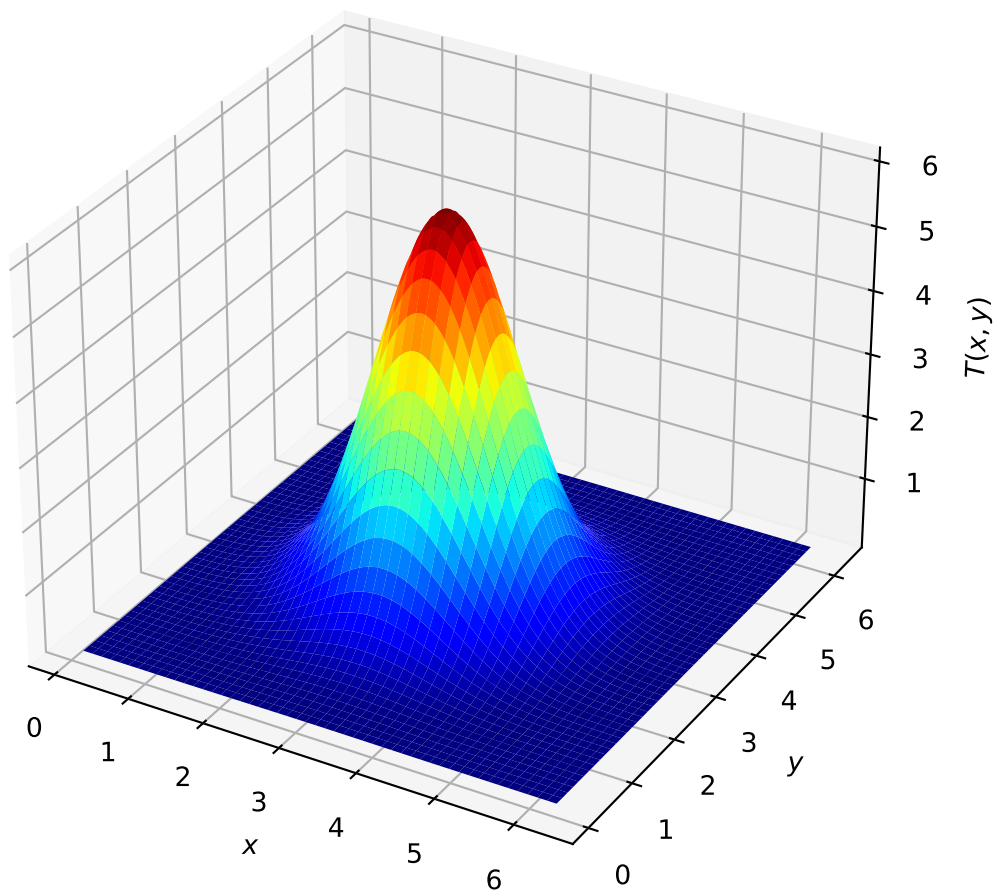
3D Plot of T(x, y) for t = 0.1
