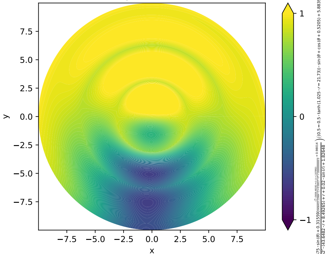
Swift-Hohenberg 2D Pattern, MSE = 0.014
