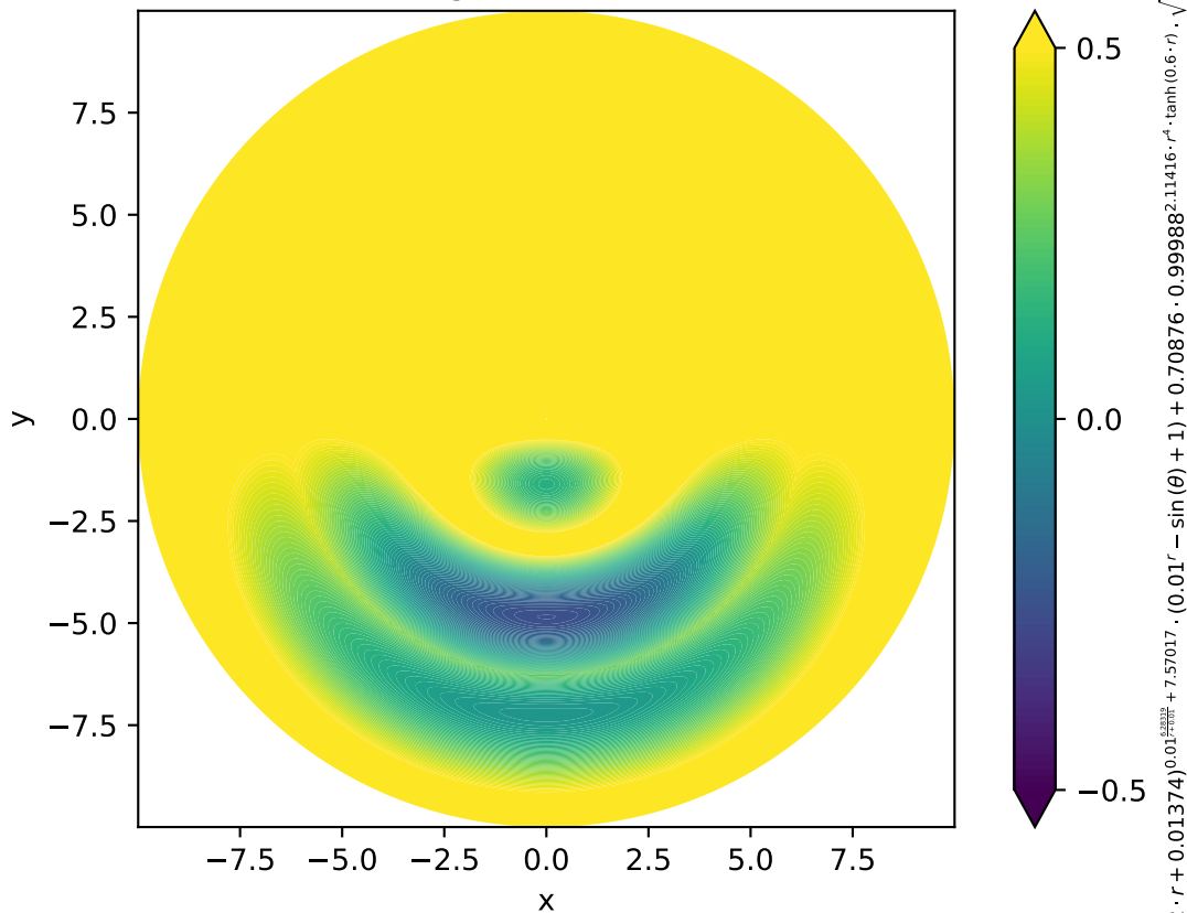
Swift-Hohenberg 2D Pattern, MSE = 0.040
