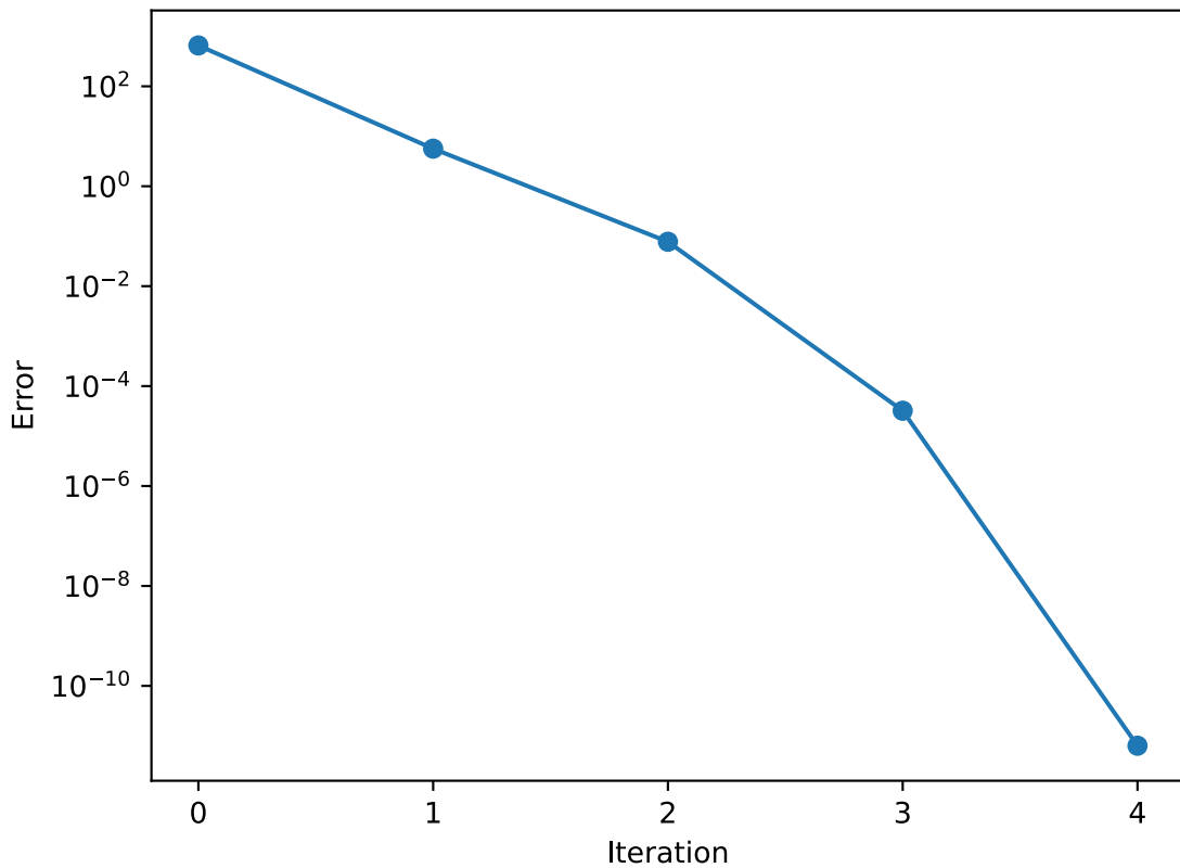
Error vs. Iterations for \varepsilon = 1
