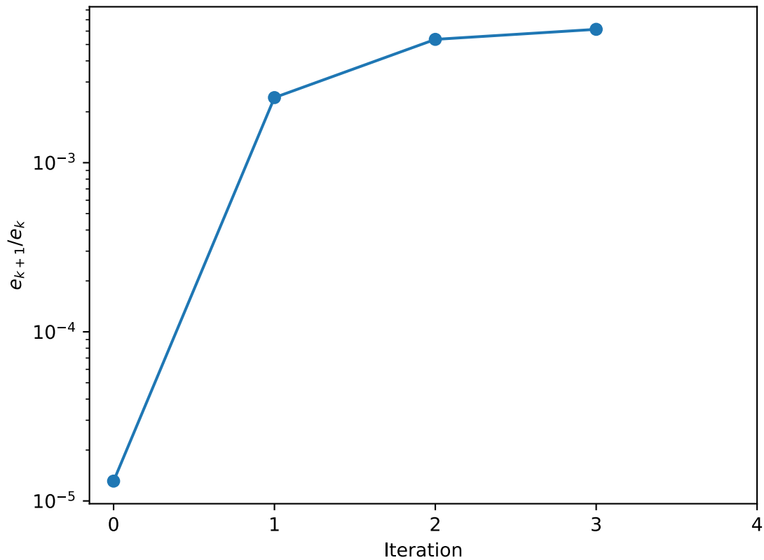
Error ratio vs. Iterations for \varepsilon = 1
