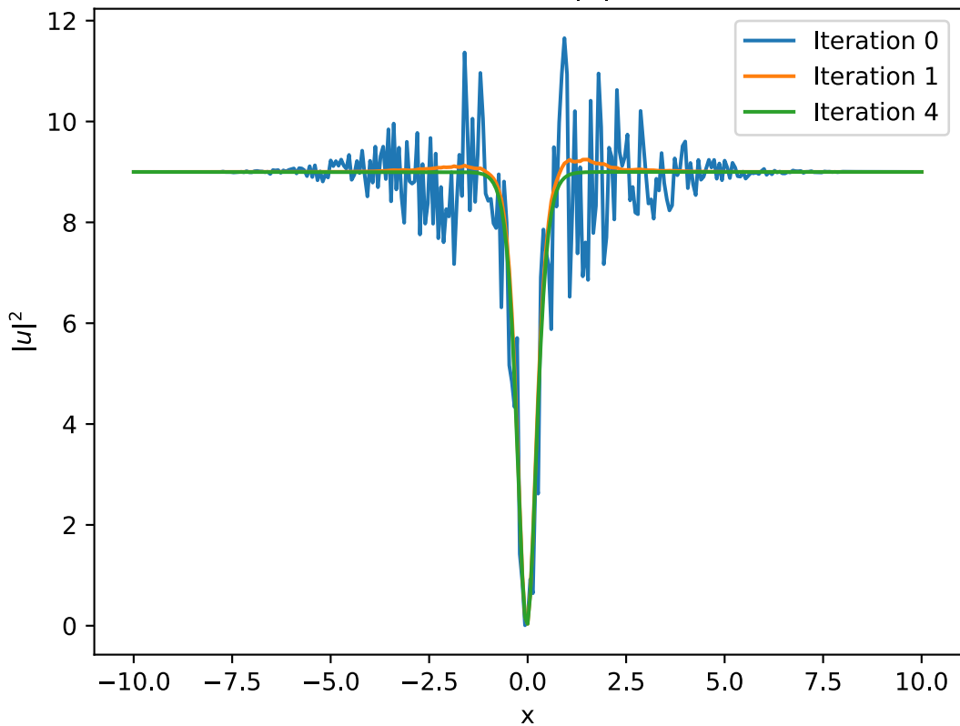
Solution Evolution |u|^2 for \varepsilon = 1
