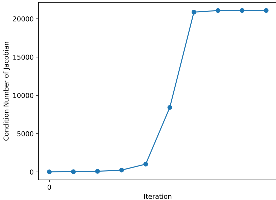
Evolution of \text{cond}(J) for \varepsilon = 1
