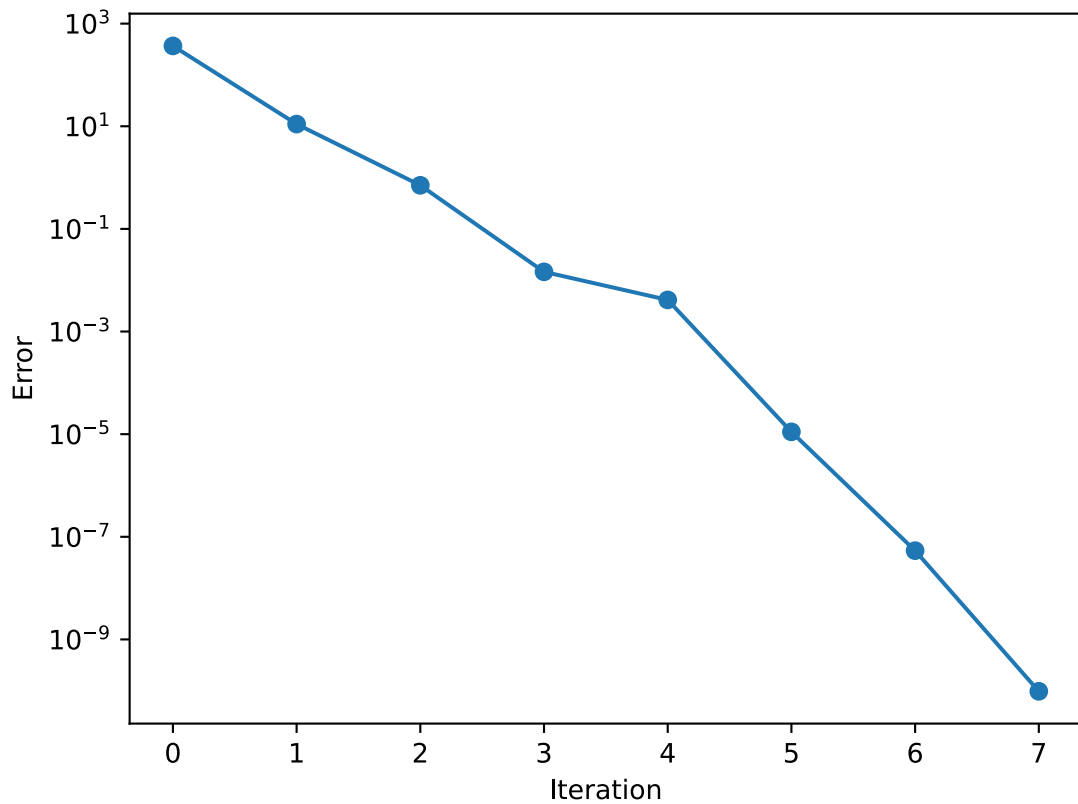
Error vs. Iterations for \varepsilon = 1
