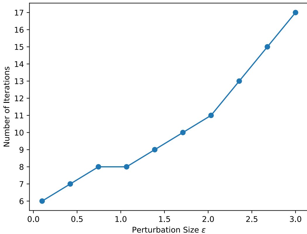
Iterations vs. Perturbation Size \varepsilon
