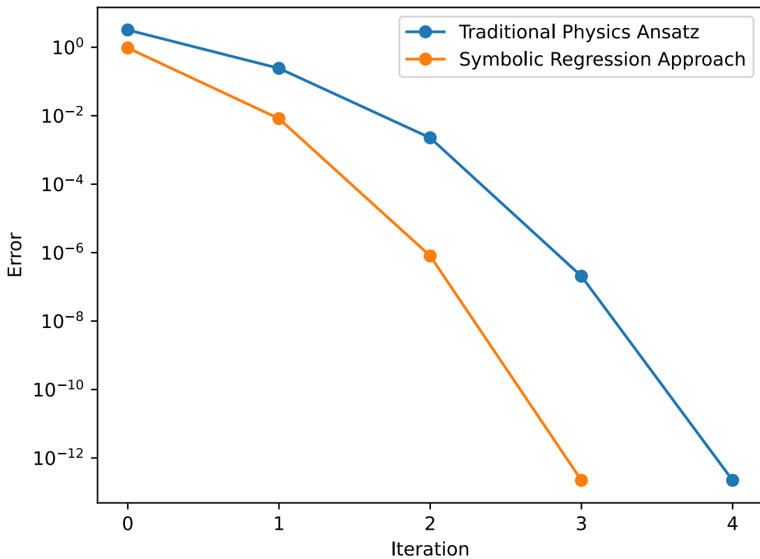
Error vs. Iterations for \varepsilon = 0
